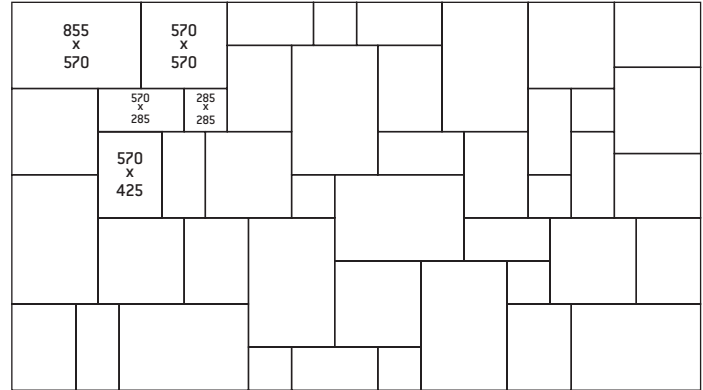
PP51 4.56 x 2.56m = 11.7m 2 Random Style
