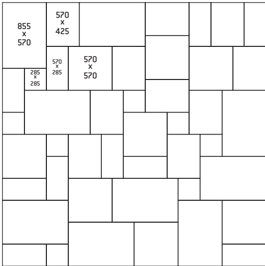
PP52 3.42 x 3.42m = 11.7m 2 Random Style
