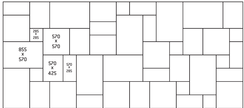
PP53 2.28 x 5.13m = 11.7m 2 Random Style
