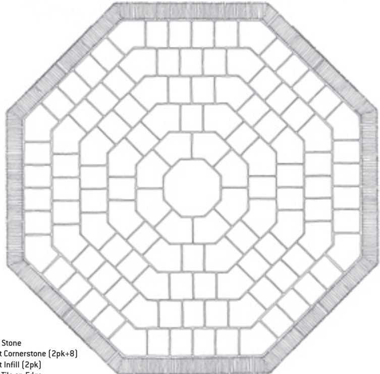
ME38 Width 3.39m Components: 1 no. Octant Centre Stone 24 no. Petite Octant Cornerstone (pk+8) 24 no. Petite Octant Infill 8 no. Octant Corner Tile on Edge 20 no. Straight Tile on Edge
