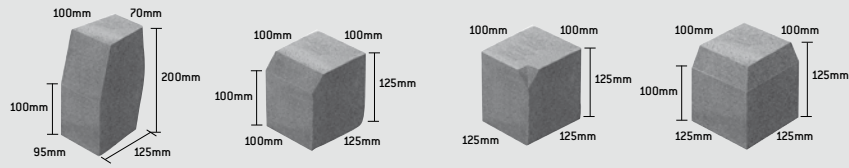
KL HB Radial
