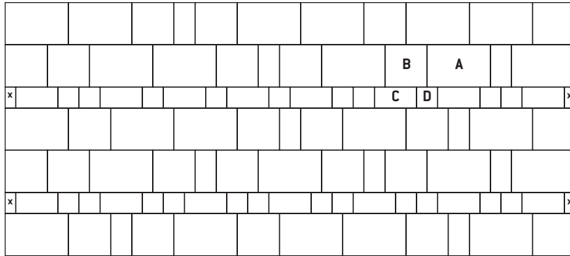
PP42 5.4 x 2.4m = 13.0m 2 Coursed Style. 2 no. 200 x 200 cut in half, where marked X
